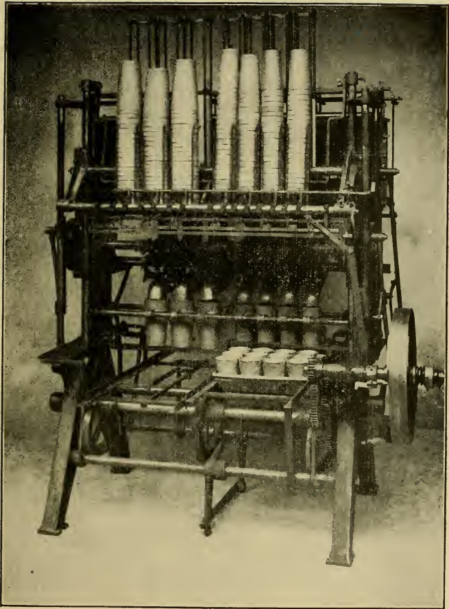
Maxwell Paper Bottle Filling and Capping Machine.
